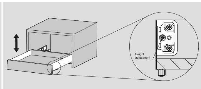
Height adjustment
