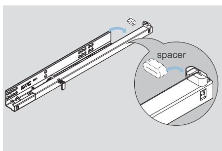
Install the spacer onto the rear hook of the slide
