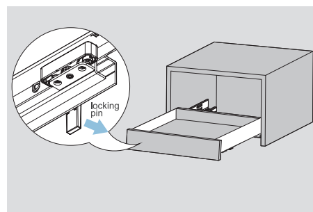
Pull out the locking pin to unlock
