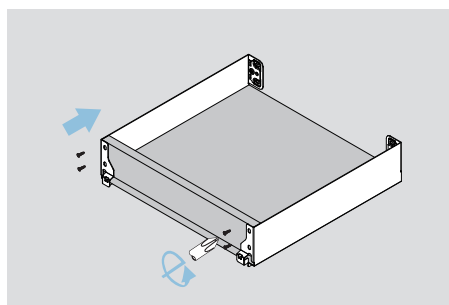
Back assembly
