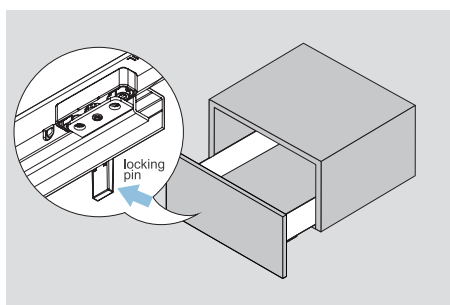
Push the locking pin to lock the side with the drawer side
