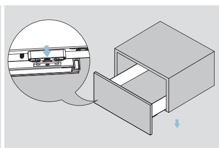
Lay the drawer onto the slide and let the peg insert into the hole under the drawer side
