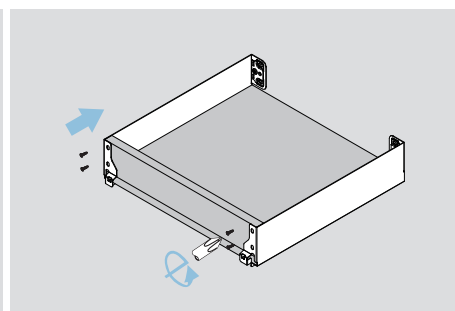
Back assembly
