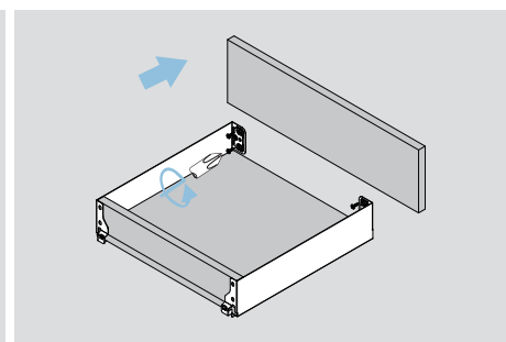
Front assembly
