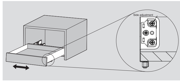
Side adjustment
