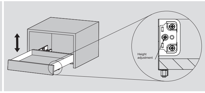
Height adjustment
