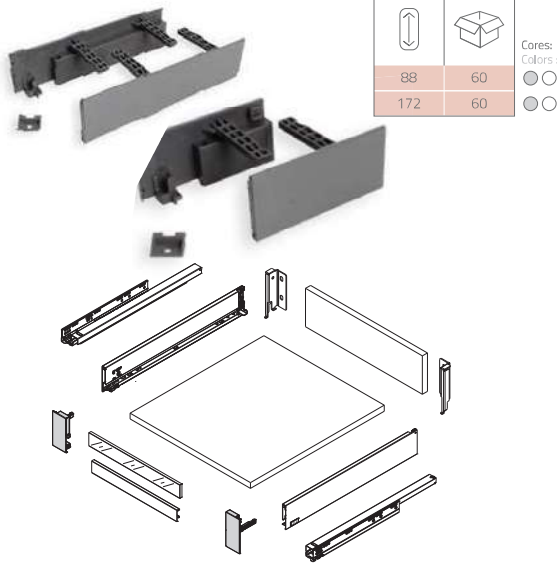
Fixador Frontal p/ Gaveta Int. de Vidro Interior Glass Drawer Front Fixer
