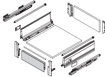
União Vareta Transv. a Vareta Lat. DTC Single DTC Cross Rail Connector to Metal Box-side
