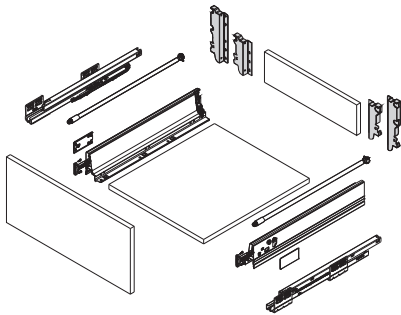
Fix. Traseiro p/ Vareta DTC DTC Side Rail Back Fixing Bracket
