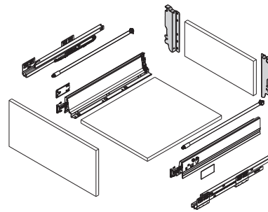
Fixador Frontal p/Vareta Quadrada DTC DTC Front Fixing Brackets to Square Rails
