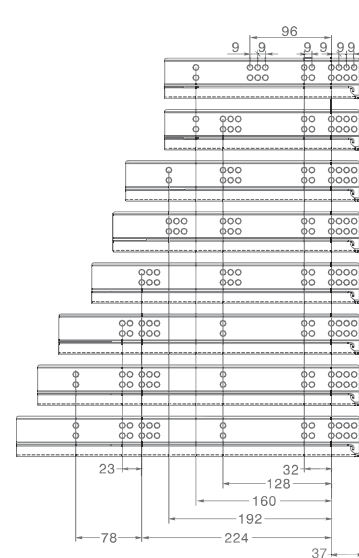
Corrediça DTC Tic-Tac Ext. Total DTC Push to Open Full Extension Slide
