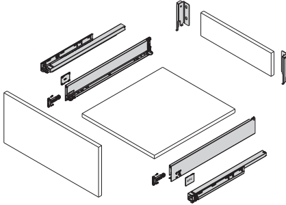
Gaveta Magic Pro 172 MM DTC DTC 172 MM Magic Pro Drawer
