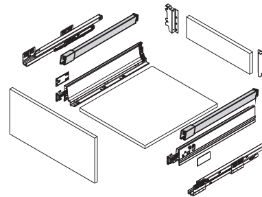
Traseiro Alto de 1 Vareta DTC DTC Back Fixing Bracket to 1 Side Rail
