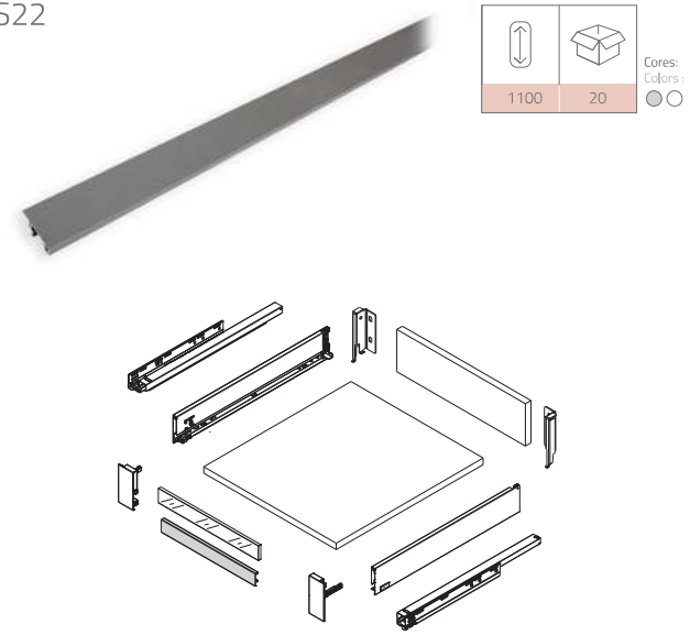
Barra Fronta p/ Gaveta Int. de Vidro Interior Glass Drawer Front Section
