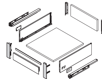
Vareta Frontal p/ Gaveta Magic Pro DTC DTC Magic Pro Drawer Cross Square Rail
