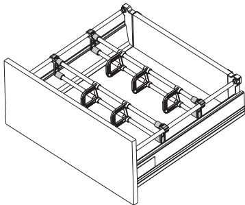
Sep. de Vareta p/Div. Dupla Transv. DTC DTC Divider on Double Cross Rail
