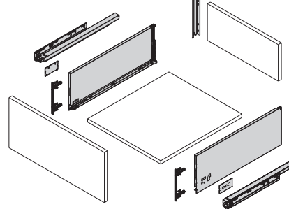
Gaveta Magic Pro 172 MM DTC c/Lateral de Vidro DTC 172 MM Magic Pro Drawer w/Glass Lateral
