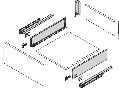
Gaveta Magic Pro 238 MM DTC DTC 238 MM Magic Pro Drawer
