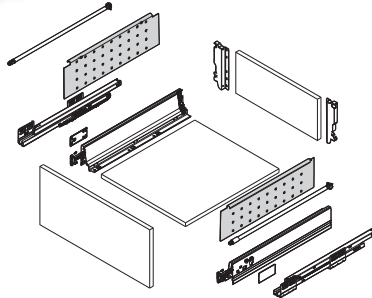
Fix. Divisória Transv. p/Painel Perf. DTC DTC Cross Divider Connector
