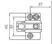
Dobradiça Articulada Articulated Hinge
